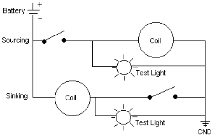
Fig 10, Sourcing and Sinking Circuits.
