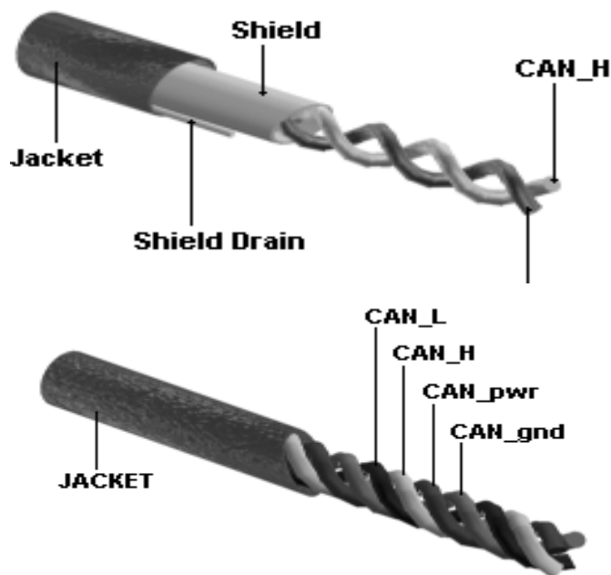
Fig. 1, CAN cables.
