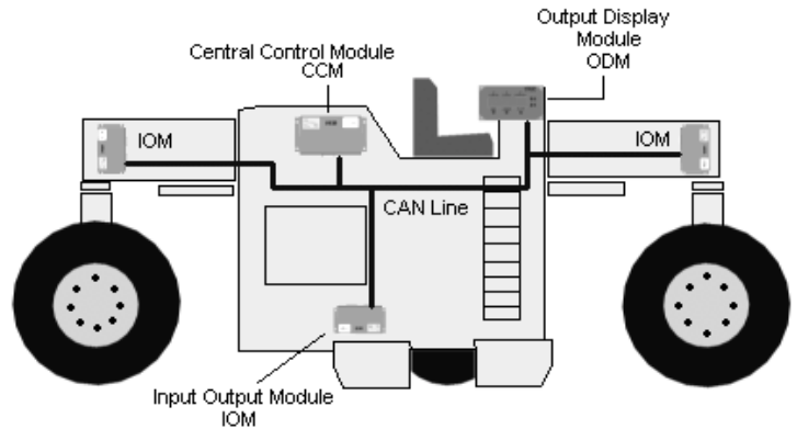
Fig 8, Road Building Machine.
