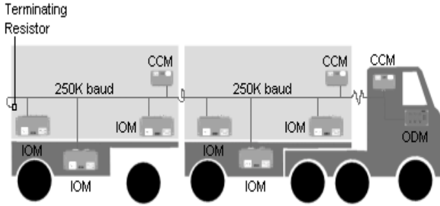
Fig 5, Tractor Trailer Application.
