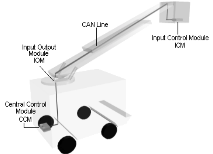
Fig 7, Aerial Work Platform Application.
