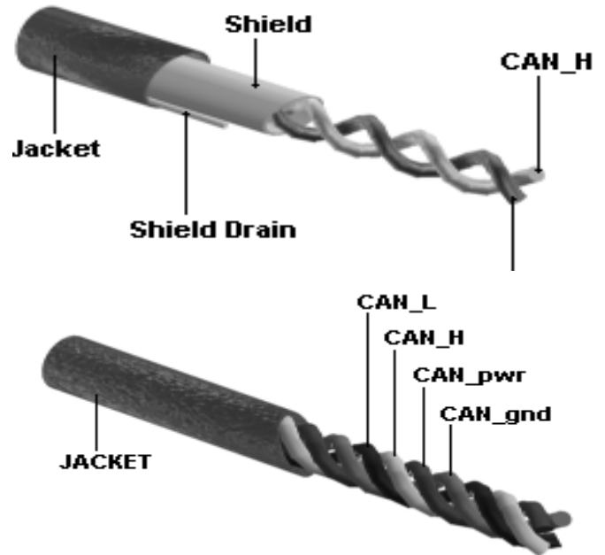
Fig. 1, CAN cables.
